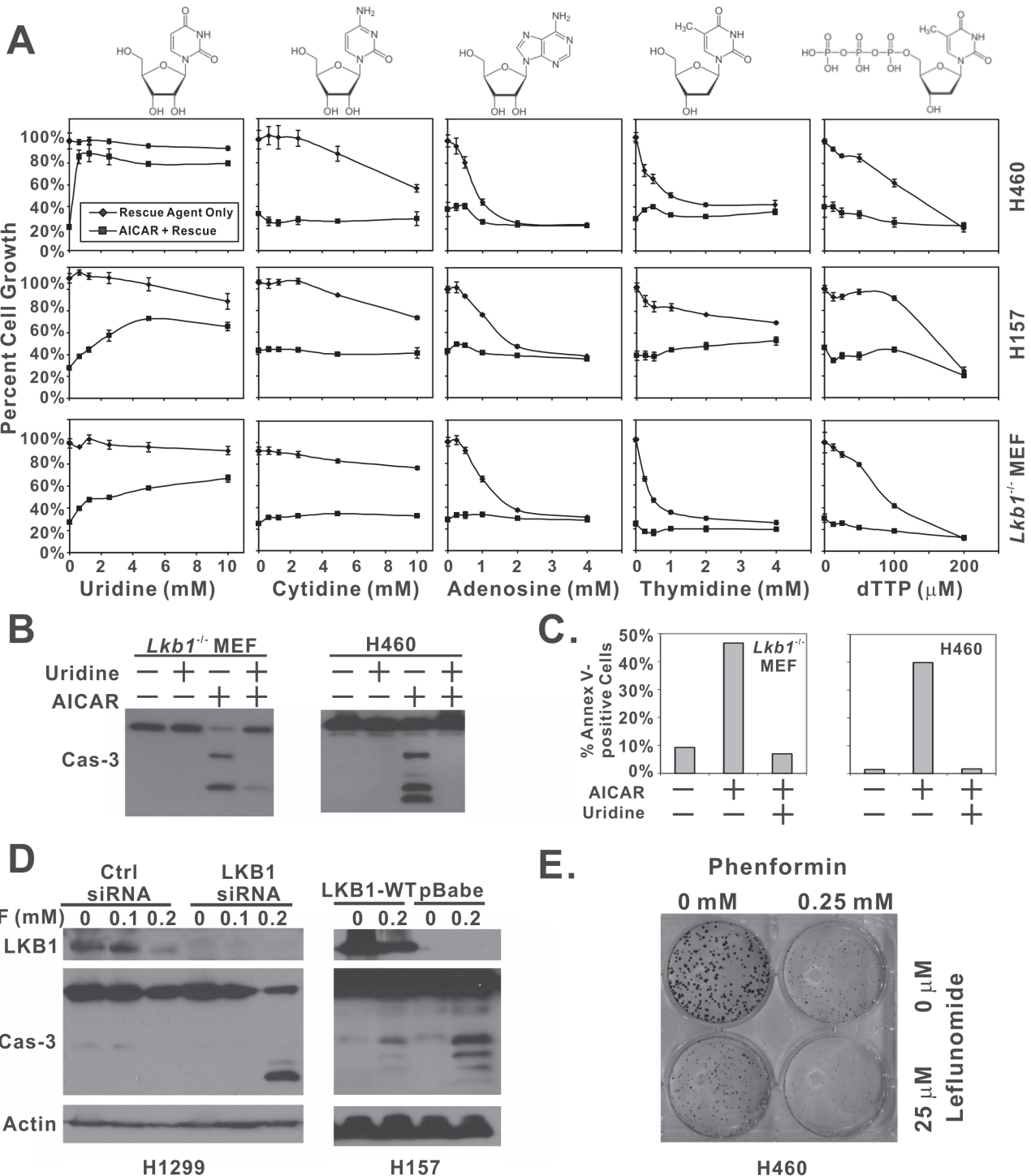
Figure 2: Depletion of uridine is responsible for AICAR-induced apoptosis in LKB1-null cells. A. H460, H157 and Lkb1 -/- MEF cells were seeded in 96-well plates, and treated with the indicated concentration of uridine, cytidine, adenosine, thymidine, dTTP alone, or their respective combination with 1 mM AICAR. Plates were subjected to SRB assay 48 hrs after treatment. Reactions were carried out in quadruplicates, and the error bars represent one standard deviation. B. Lkb1 -/- MEF and H460 cells were seeded in 6-well plates and treated with 1 mM AICAR alone, 5 mM uridine alone or their combination. Lysates were collected 24 hrs after treatment for immunoblot analysis of total caspase-3. C. For Annexin-V and 7AAD analysis of apoptosis, Lkb1 -/- MEF and H460 cells were seeded in 6-well plates, and treated with 1 mM AICAR alone, 5 mM uridine alone, or their combination. Both floating and attached cells were collected 24 hrs after treatment and subjected to flow analysis. Percentage of Annexin-V positive cells was reported. D. Isogenic H157-pBabe and H157-LKB1-WT cells were treated with 0.2 mM of leflunomide for 48 hrs. Cell lysates were collected and analyzed by immunoblot with indicated antibodies. LKB1 was depleted in H1299 cells by siRNA and treated with 0, 0.1, or 0.2 mM of leflunomide for 48 hrs. Cell lysates were collected for immunoblot of LKB1 and total caspase-3. E. H460 cells were treated with 0.25 mM phenformin, 25 μM leflunomide, or their combination for 10 days in a colony formation assay.
