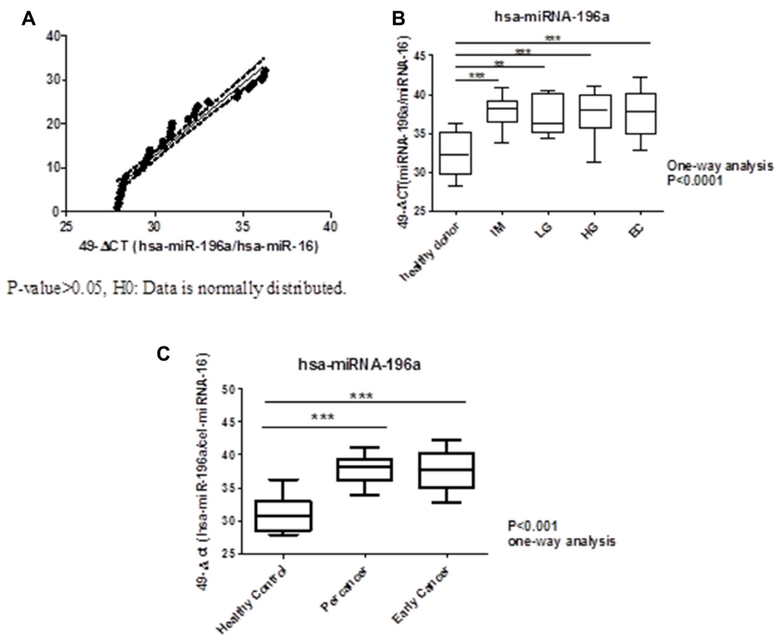
Figure 1: Normality test for healthy volunteers and boxplots of expression of miRNA196a in plasma. ***P-value < 0.001 **P-value < 0.01. (A) Normality Test for Healthy Control. (B) Boxplots of Expression of miRNA-196a in Plasma for healthy donor (control), all stages of precancer and early cancer. (C) Boxplots of Expression of miRNA-196a in Plasma for healthy control, precancer, and early cancer. IM: intestinal metaplasia; LG: low-grade dysplasia; HG: high-grade dysplasia; EC: early cancer.
