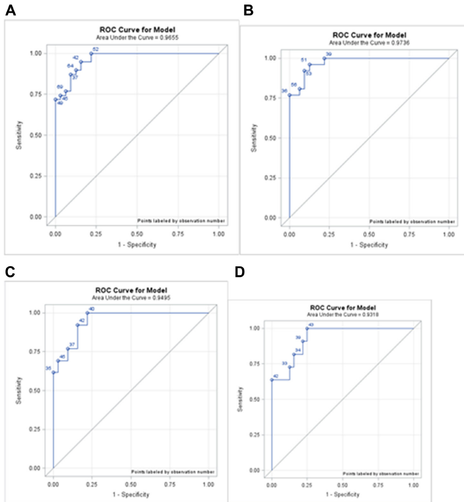
Figure 2: ROC curves for each phase. (A) ROC curve of healthy subjects vs. IM, HGD, and LGD; AUC was 0.9655. (B) ROC curve of healthy subjects vs. IM; AUC was 0.9736. (C) ROC curve of healthy subjects vs. LGD and HGD; AUC was 0.9495. (D) ROC curve of healthy subjects vs. EC; AUC was 0.9318. IM: intestinal metaplasia; LGD: low-grade dysplasia; HGD: high-grade dysplasia; EC: early cancer.
