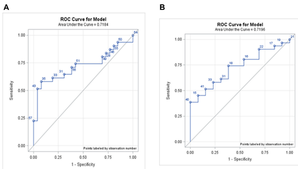
Figure 3: ROC curves for each phase. (A) ROC curve of IM vs. EC; AUC was 0.7184. (B) ROC curve of LGD/HGD, vs. EC; AUC was 0.7196. IM: intestinal metaplasia; LGD: low-grade dysplasia; HGD: high-grade dysplasia; EC: early cancer.
