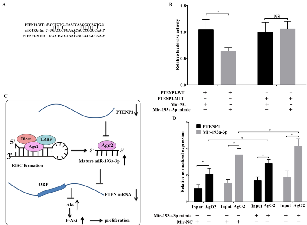
Figure 4: PTENP1 as a sponge directly interacted with miR-193a-3p. (A) and (B) The binding sequence was predicted by FindTar3 online. The wild type and mutant PTENP1 sequences were cloned into pMir-Reporter vectors and co-transfected with miR-193a-3p mimic or miR-NC into SMMC-7721 cells. Then, the dual luciferase activity was detected. (C) Schematic of the proposed mechanism of PTENP1 in HCC cells. PTENP1 as a sponge interacted with miR-193a-3p and modulated the expression of PTEN/Akt pathway, leading to repress cells proliferation in HCC. (D) RNA immunoprecipitation with the anti-Ago2 antibody was applied to evaluate endogenous Ago2 binding to RNA. The levels of PTENP1 and miR-193a-3p were analyzed by qPCR from Ago2 precipitate. Data was expressed as means \pm SD, n=3. *P < 0.05, NS: no significance.
