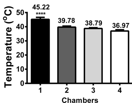
Figure 2: The formation of a stable temperature gradient from 37°C to 45°C. The stable temperature gradient was recorded from 37°C to 45°C when chamber 1 was heated to 45°C.
