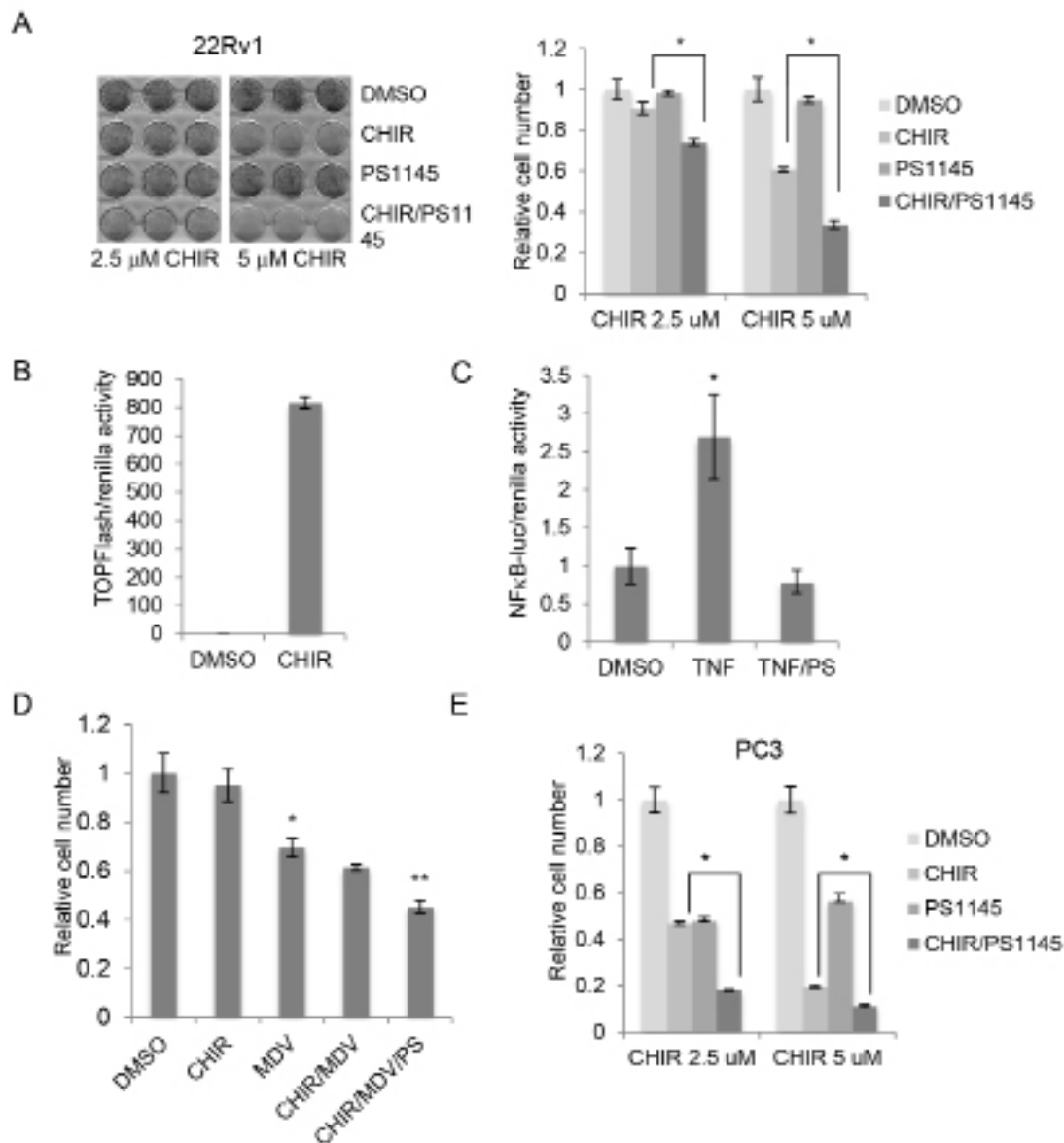
Figure 4: Inhibition of NFκB potentiates the inhibitory effect of CHIR99021 on PCa cell proliferation. (A) Left: representative experiment showing crystal violet staining of 22Rv1 cells cultured for 1 week with DMSO, 10 \mu M PS1145 and/or the indicated concentrations of CHIR99021 (CHIR). Right: absorbance (540 nm) of solubilized crystal violet was used to calculate relative cell number; * p < 0.01 . (B) \beta -catenin/Tcf-dependent transcriptional activity in 22Rv1 cells treated with carrier (DMSO) or 5 \mu M CHIR99021 (CHIR) was determined by gene reporter assay using Super8xTOPFlash normalized to renilla. (C) NFκB-dependent transcriptional activity in 22Rv1 cells treated with carrier or TNF and 10 \mu M PS1145 (PS) as determined by gene reporter assay using NFκB-luciferase normalized to renilla; * p < 0.01 vs. DMSO. (D) Quantitation of crystal violet assays showing relative cell number for 22Rv1 cells cultured for 1 week in the presence of carrier (DMSO) +/- 1 \mu M CHIR99021 (CHIR), 10 \mu M MDV3310 (MDV) and 10 \mu M PS1145 (PS); p < 0.05 versus DMSO (*) and versus MDV (**). (E) Quantitation of crystal violet assays showing relative cell number for PC3 cells cultured for 1 week in the presence of DMSO, 10 \mu M PS1145 and/or the indicated concentrations of CHIR99021 (CHIR); * p < 0.01 .
